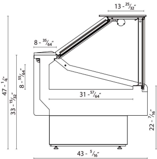
Standard Mounting
