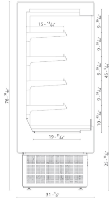
Optional Mounting
