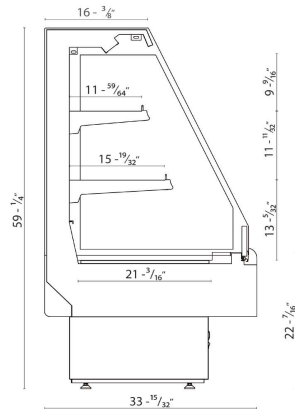
Standard Mounting
