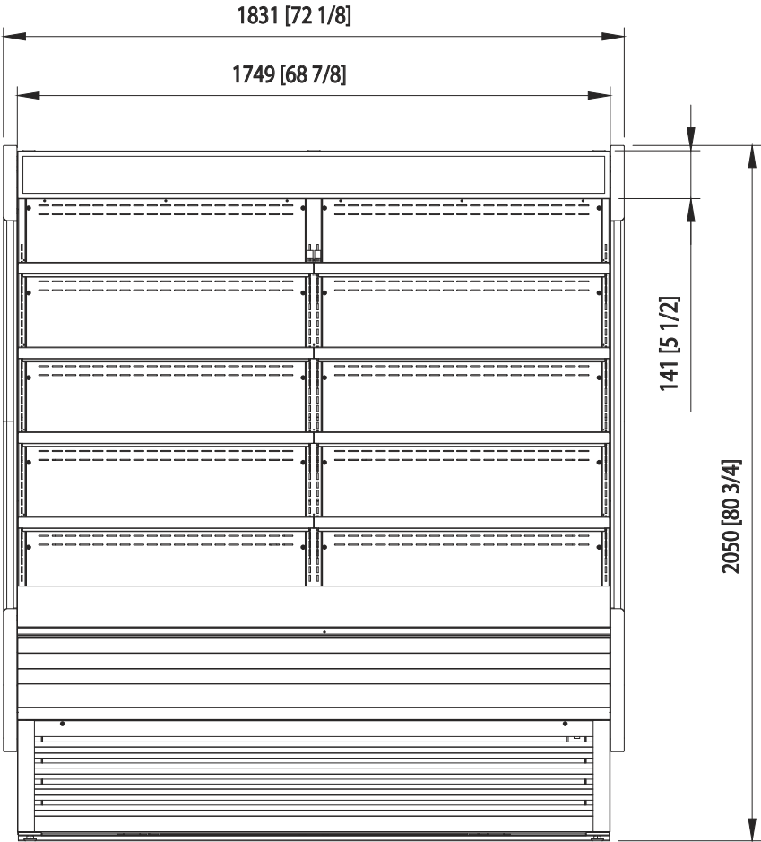
Front view
