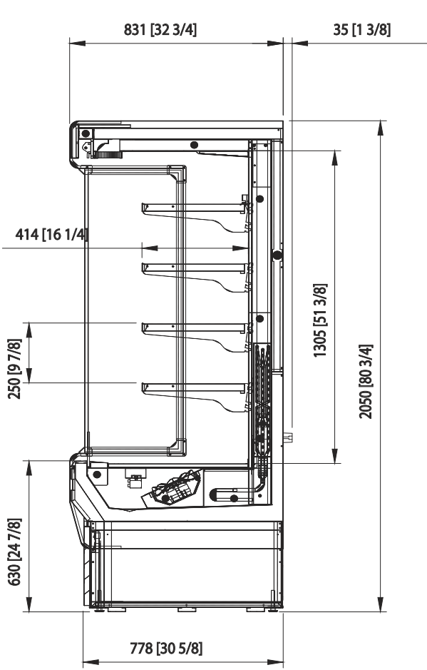
Side view
